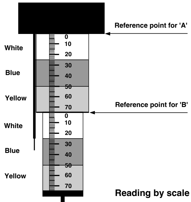
Figure 2 Cablebolt dual height tell-tale reading methods
