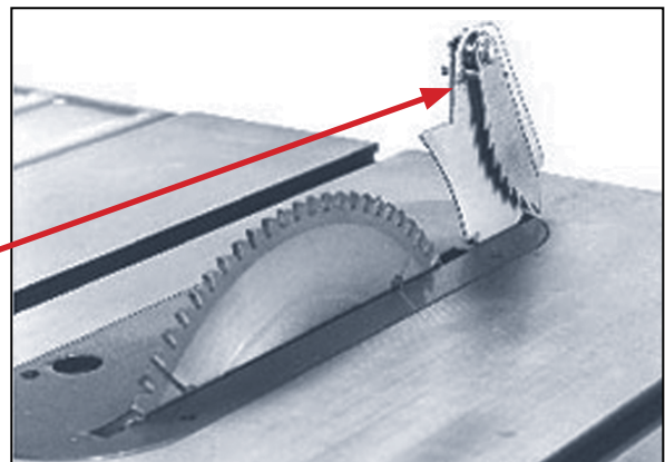
Biesemeyer Products/Delta Machinery Guard removed to show spreader device.
