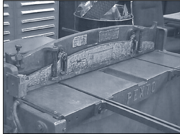
Adjustable barrier-type guard.
