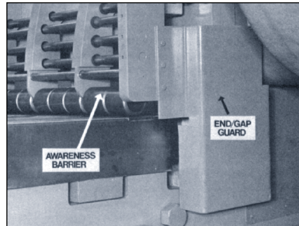
If the C-frame throat is open on either side of a power squaring shear, the gap must be guarded.
